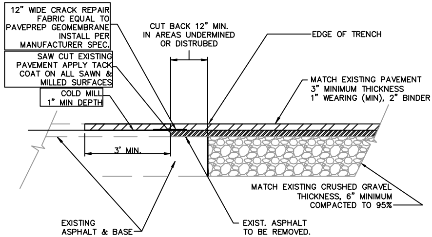
TRENCH CROSS SECTION DETAIL
