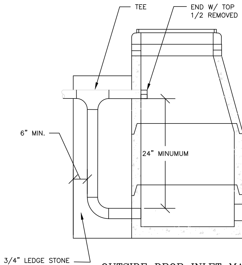
OUTSIDE DROP INLET MANHOLE FOR DROP GREATER THAN 2' & ID < 5'
