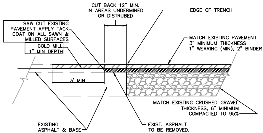
TRENCH CROSS SECTION DETAIL
