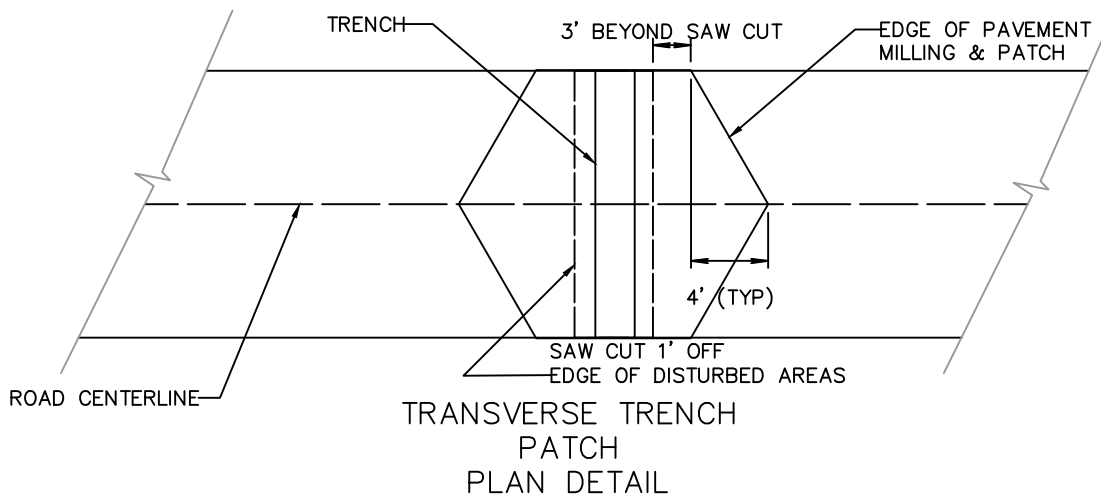
SINGLE LANE TRENCH PATCH PLAN DETAIL
