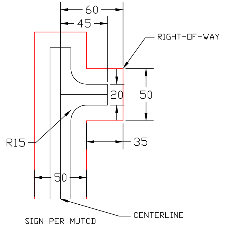
HAMMERHEAD CUL-DE-SAC
