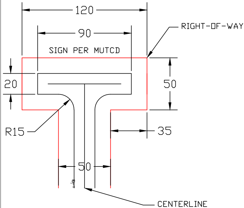
HAMMERHEAD CUL-DE-SAC
